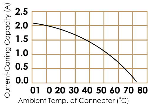
Figure 2: Current Rating
