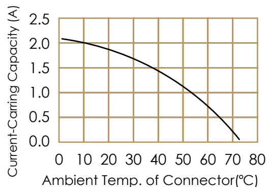
Figure 2 : Current Rating
